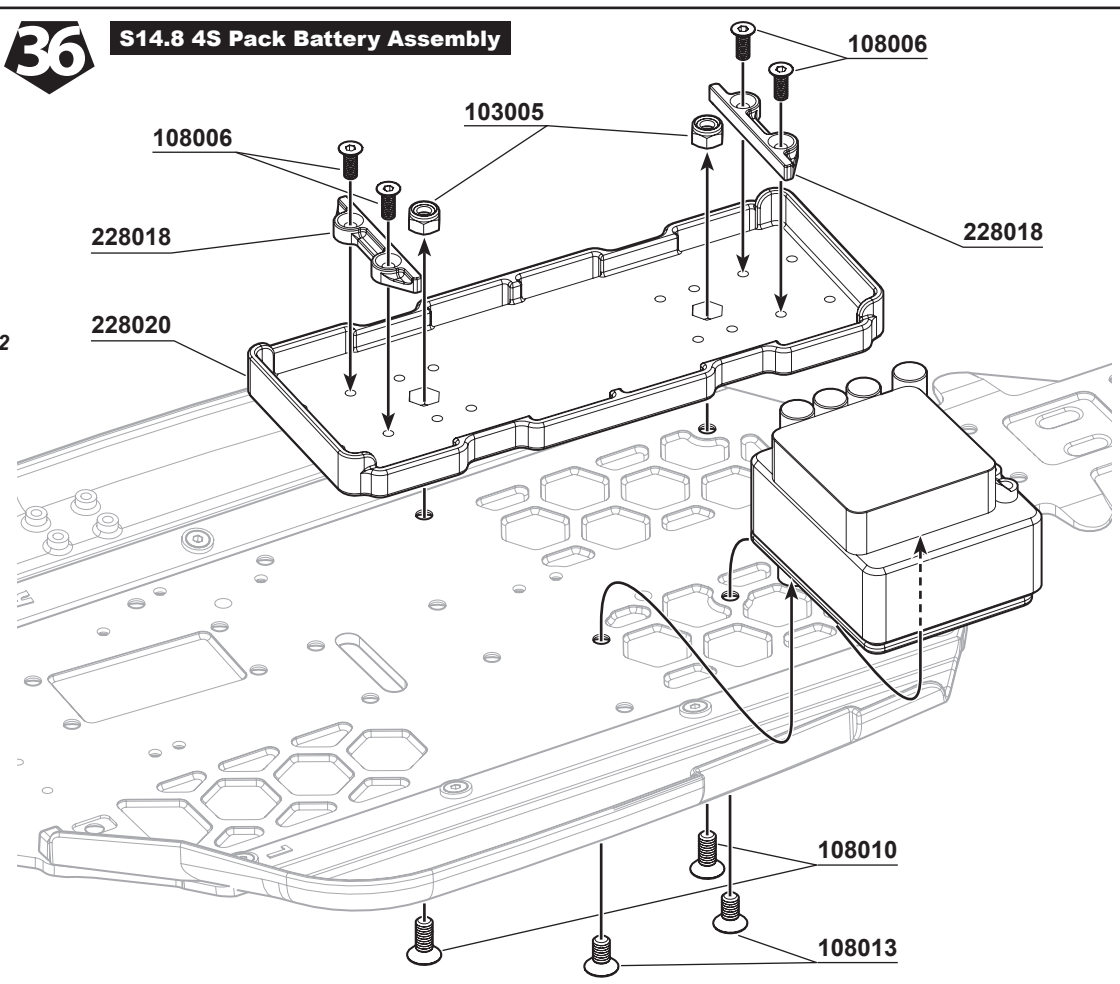
108006 M3x8mm FH/ST HEX Screw x4
