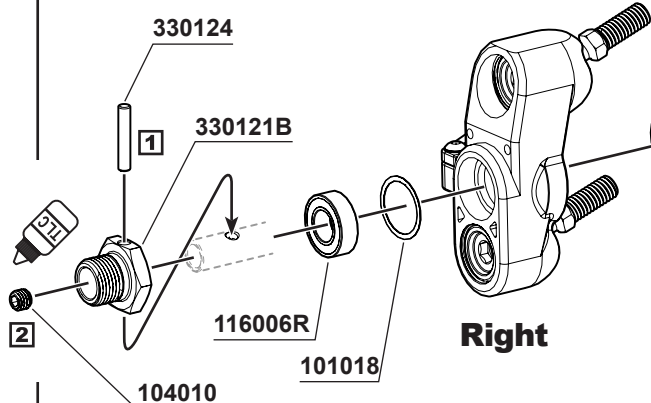
101018 SHIM 13x16x0.2mm x2
