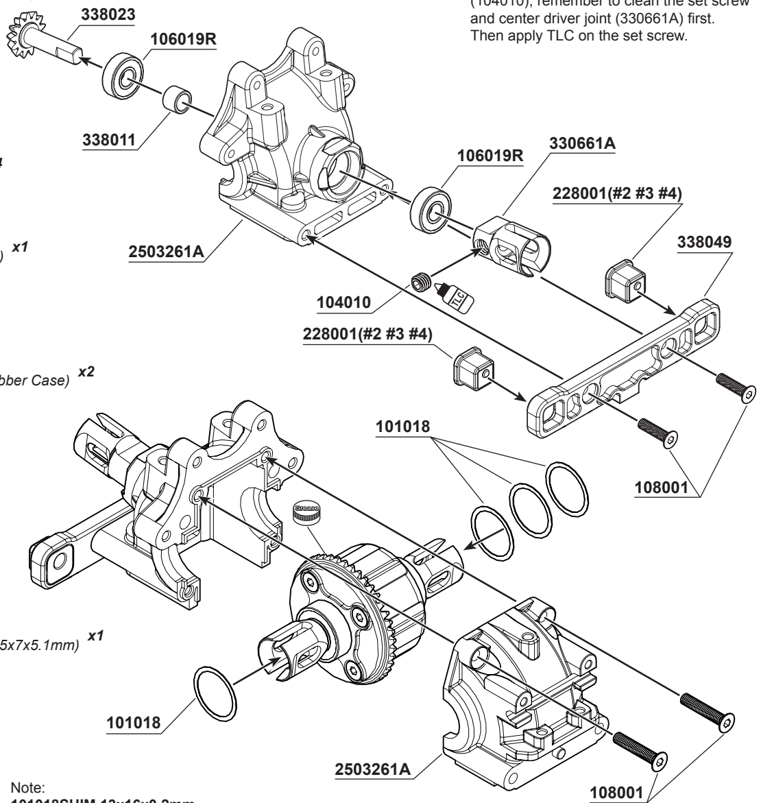
108001 M3x12mm FH/ST HEX Screw x4
