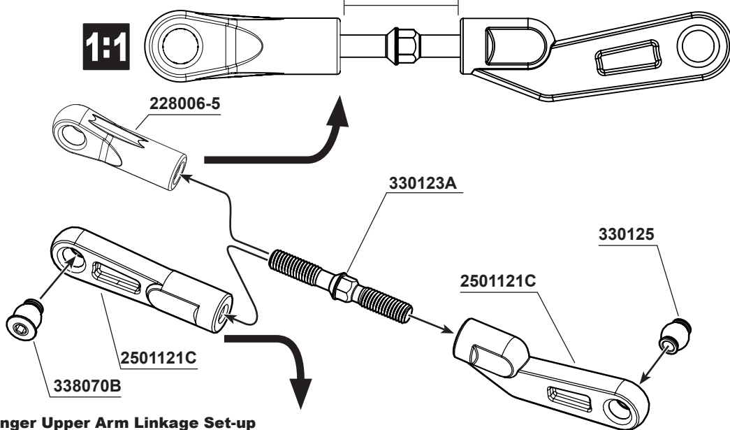
330123A Rear Upper Sus. Arm Turnbuckles x2
