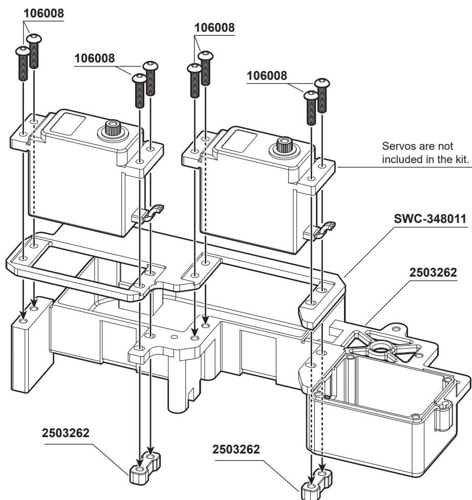
106008 M3x12mm Hex Socket OH/TP Screw x8
